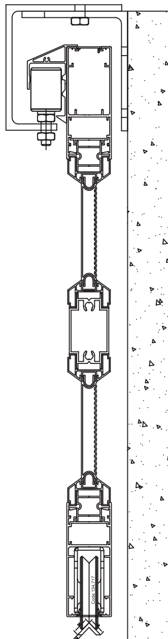
SLIDING GATE
