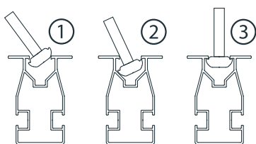
Ways of inserting aluminum nut in the profile
