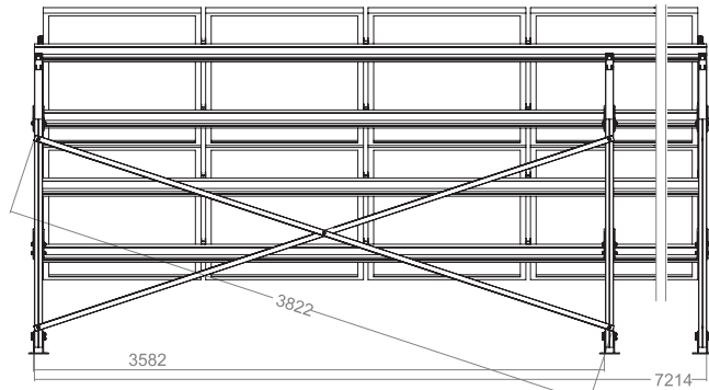
Back view of a triangle in 2 Portrait layout Izgled zadnjeg dela fotonaponskih panela
