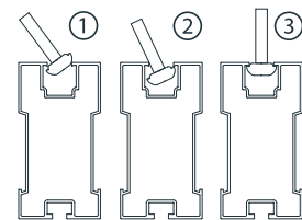
How to insert the nut in the profile Kako montirati maticu u profil
