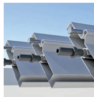
Plastic axle (Polyamide 6) offers stability, resistance and noiseless movement.
