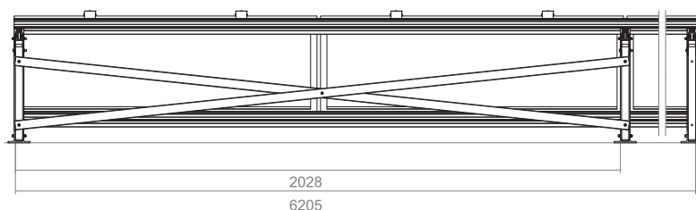
Back view of a triangle in 1 Landscape layout Presek zadnjeg dela fotonaponskog panela
