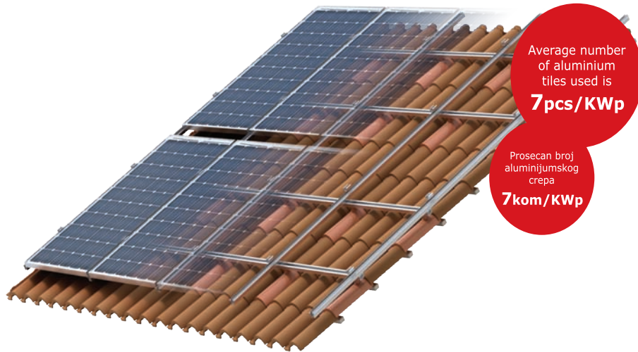
Installation steps for a double layout aluminium roof tile Montiranje duple vertikalne sa aluminijumskim crepom
