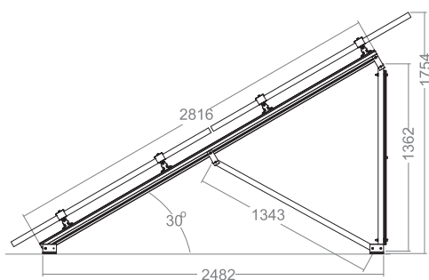
Side view of a triangle in 2 Portrait layout Bočni presek fotonaponskog panela
