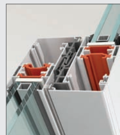
Detail of double overlapping door.
