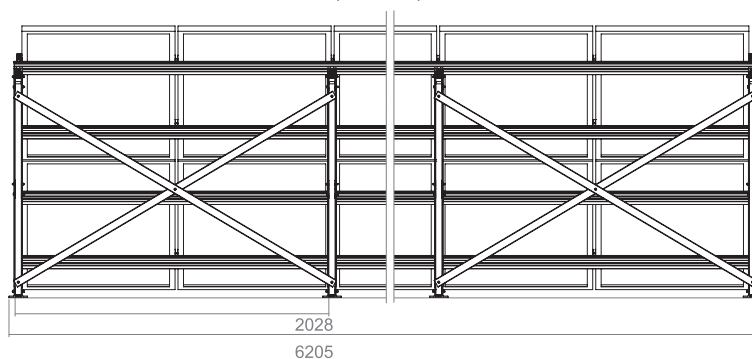
Back view of a triangle in 2 Portrait layout Presek zadnjeg dela fotonaponskih panela
