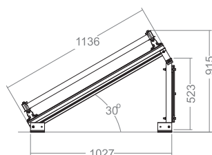
Side view of a triangle in 1 Landscape layout Bočni presek fotonaponskog panela
